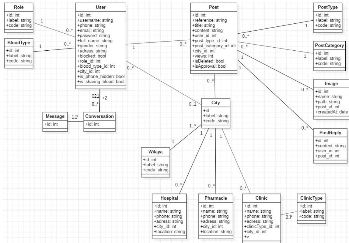
Figure 21: Class Diagram
