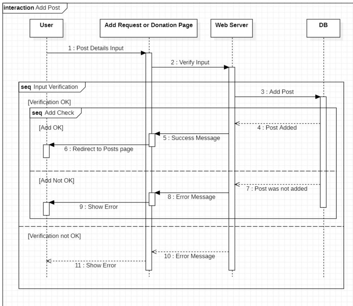
Figure 17: Add Post Sequence Diagram
