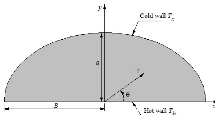
Fig. 1. Schematic presentation of the physical model
