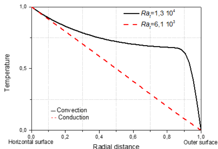
Fig. 4. Temperature distribution
