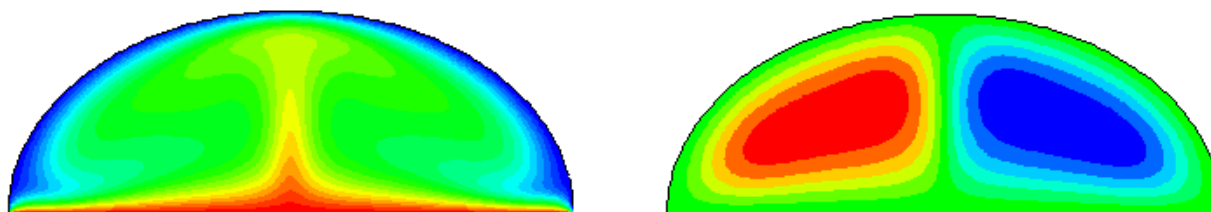
6. Isotherms and streamlines for Ra_t = 3.1 \cdot 10^5
