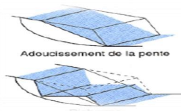
Figure 1.10 : Reprofilage
