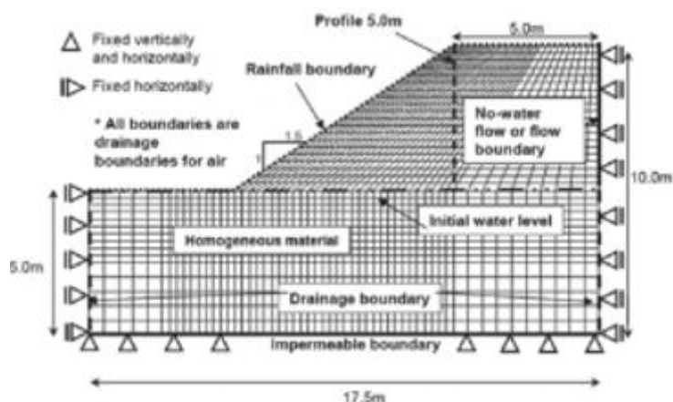
Figure II.1 : maillage et conditions aux limites
