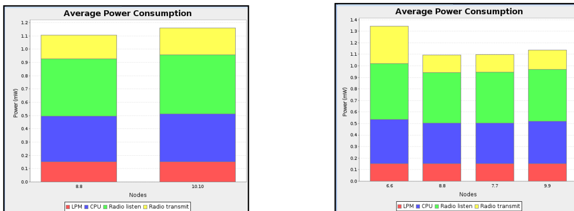
6 Sink 4 Nodes
