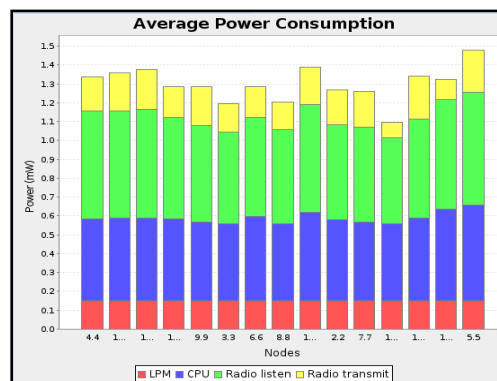
1 Sink 15 Nodes
