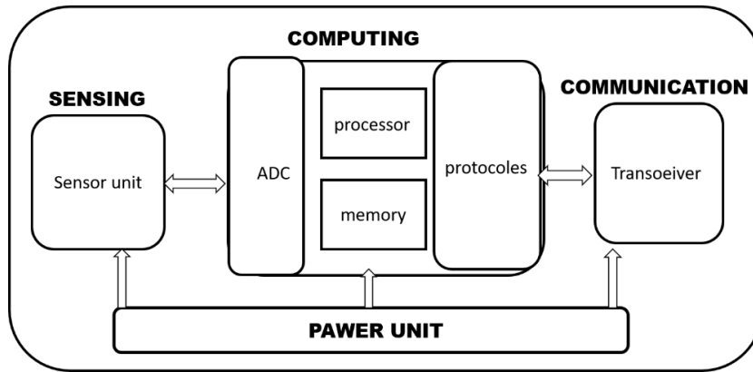
Figure2. sensor-node architecture.
