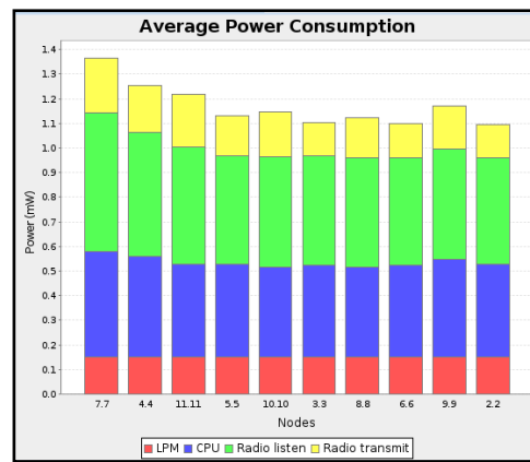
1 Sink 10 Nodes
