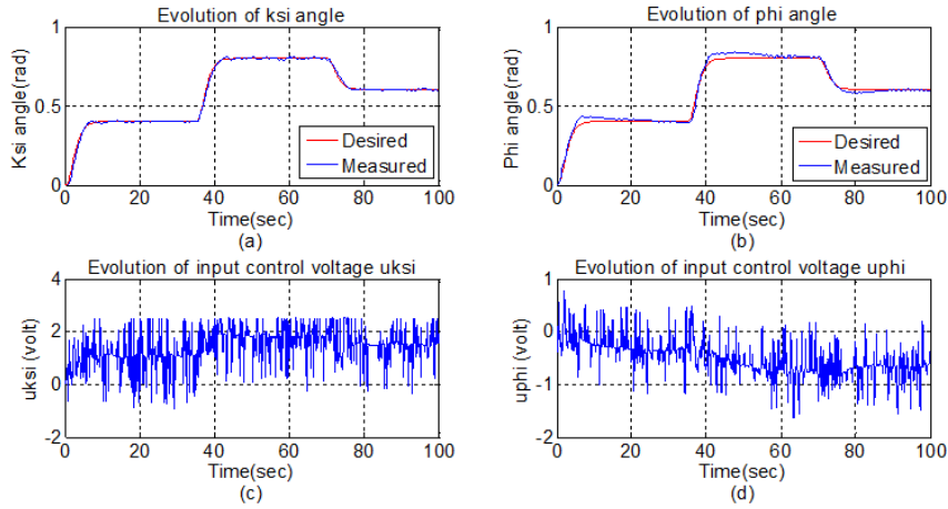
Figure 17. Experimental results of the square signal tracking
