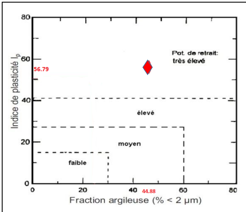
Figure III-37: Classification du sol étudié (Building Research Establishment (1980)).
