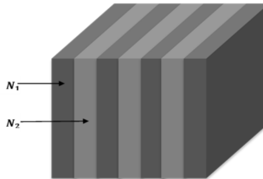
Figure II.4 Structure périodique 1D.
